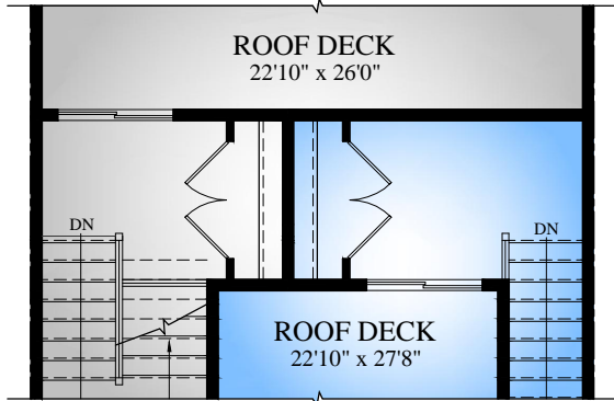
PARTIAL ROOF DECK PLAN AT PILOT HOUSE OPTION #1
