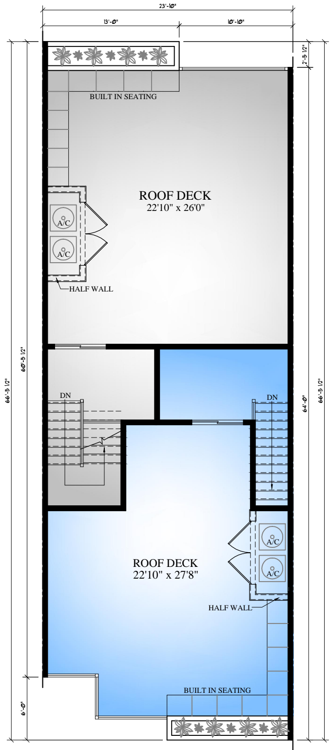
ROOF DECK FLOOR PLAN 8'0" CEILING HEIGHT
