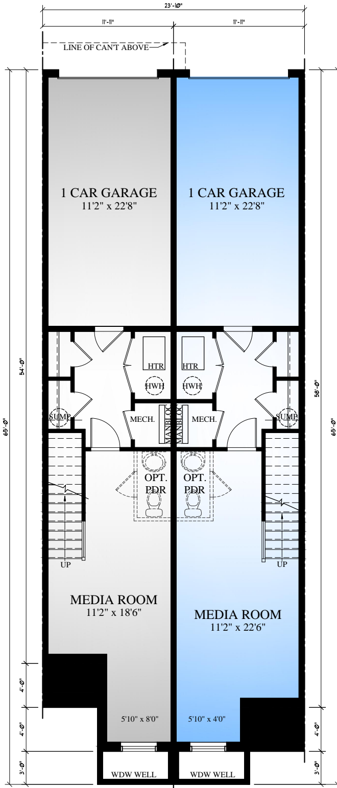
BASEMENT FLOOR PLAN 9'0" FOUNDATION WALL HEIGHT
