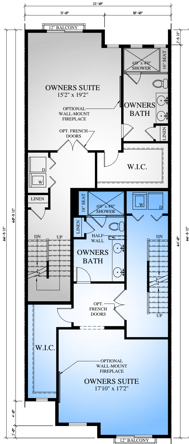
SECOND FLOOR PLAN 8'0" CEILING HEIGHT
